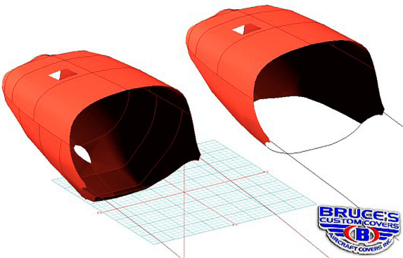
Lancair IV-P Insulated Engine Cover, fully enclosed Lancair Insulated Engine Covers, fully and partially enclosed, 3D models
